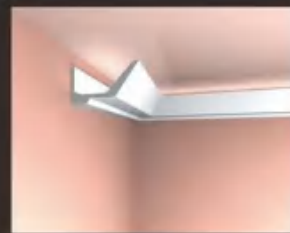
150mm 80mm HN-86220* 长度 (Long) :2440mm
